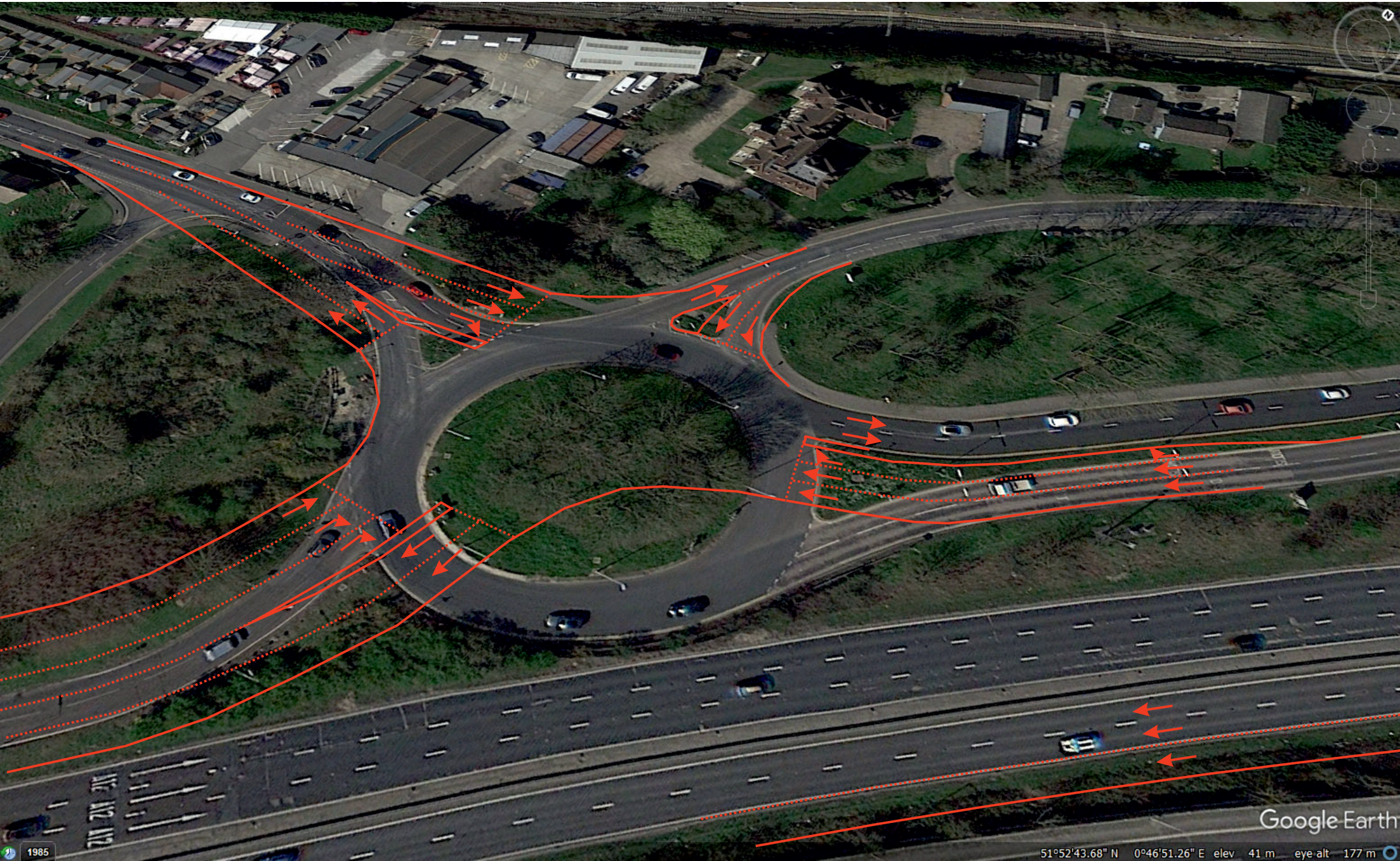
A12 Widening - Marks Tey Old Rectory Junction - Existing and Proposed
